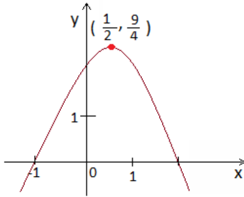
Graph of f(x) = -x^2 + x + 2
